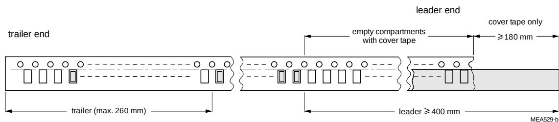
Fig. 6 Leader/trailer tape
