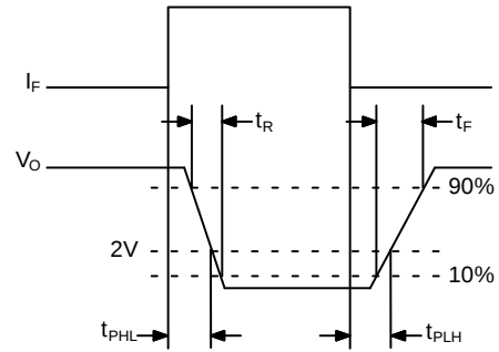
Figure 16. Timing Diagram
