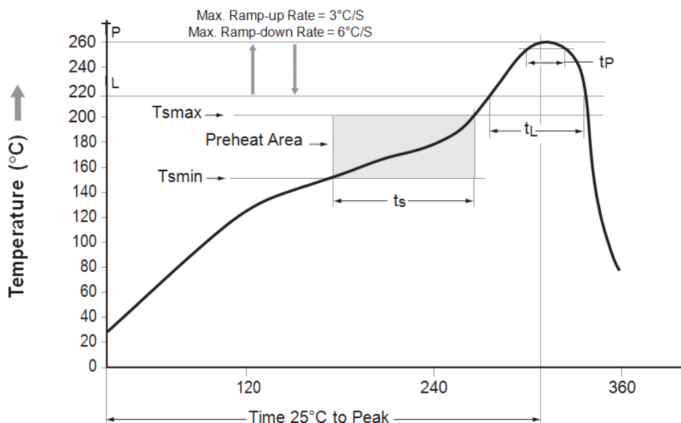
Figure 17. Reflow Profile
