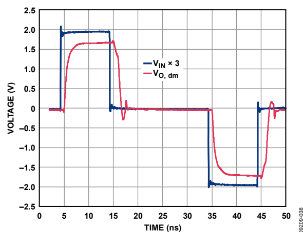
Figure 38. V_{\text{O, dm}} Overdrive Recovery
