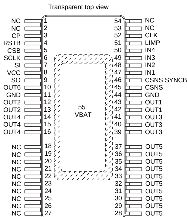
Figure 3. Pinout Diagram
