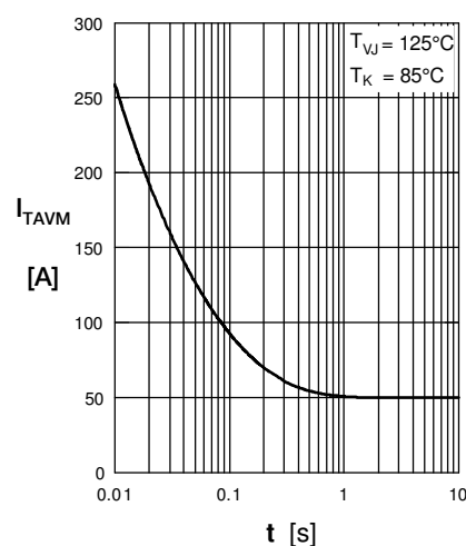
Fig. 8 Rated RMS current vs. time (360° conduction)
