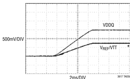
External Start-Up
