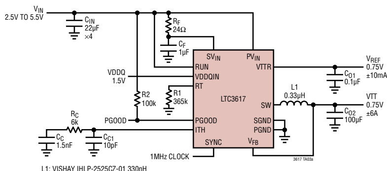
0.75V, \pm 6A DDR Termination Using a 1MHz External Clock
