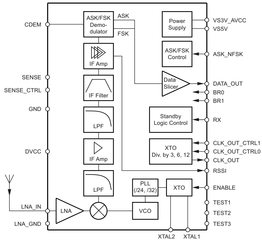
Figure 1-3. Block Diagram
