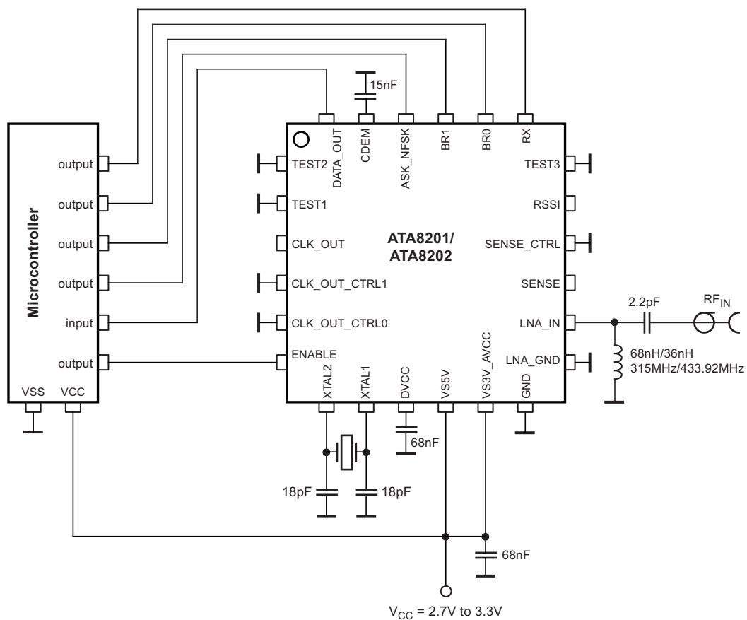
Figure 9-1. 3V Application
