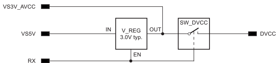
Figure 5-1. Power Supply
