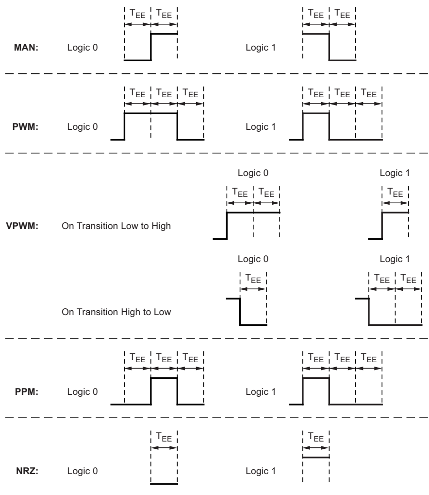
Figure 6-1. Examples of Supported Modulation Formats
