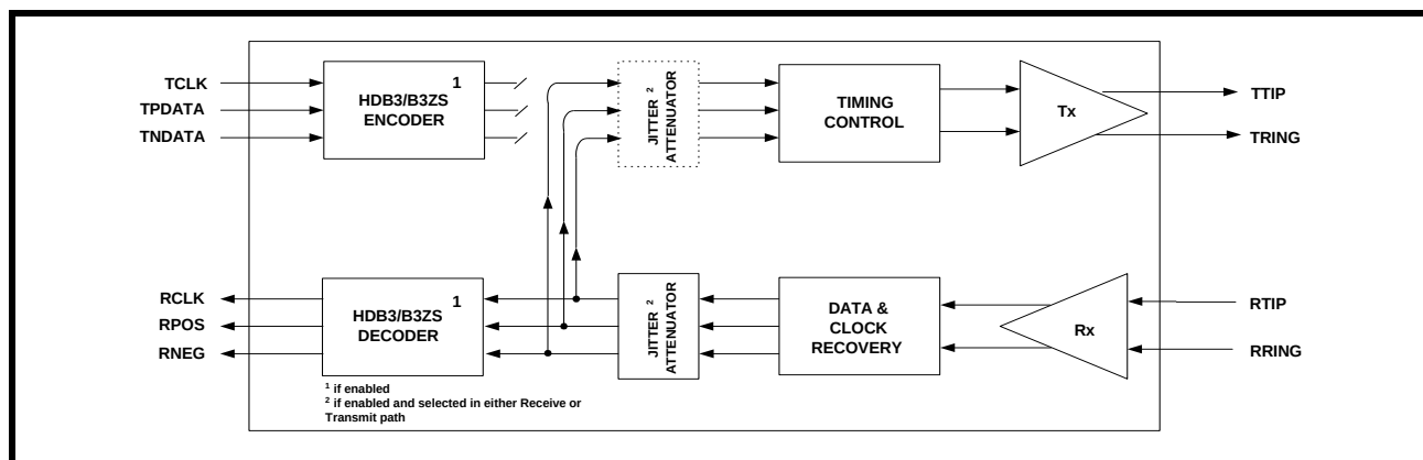
FIGURE 28. REMOTE LOOPBACK
