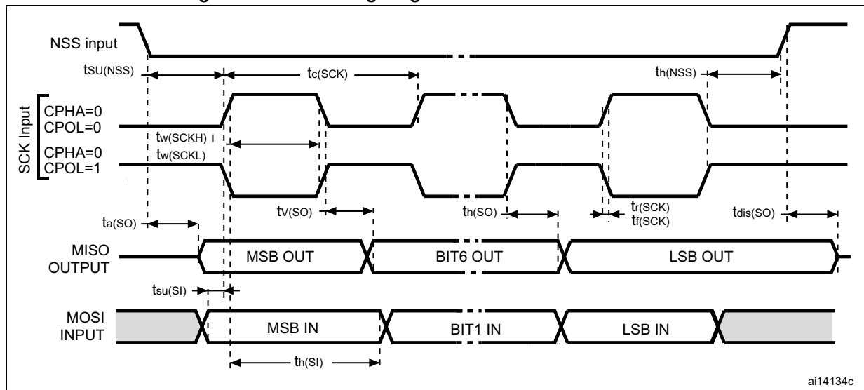
Figure 39. SPI1 timing diagram - slave mode and CPHA=0
