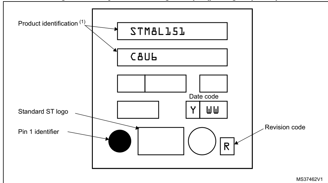
Figure 59. UFQFPN48 marking example (package top view)
