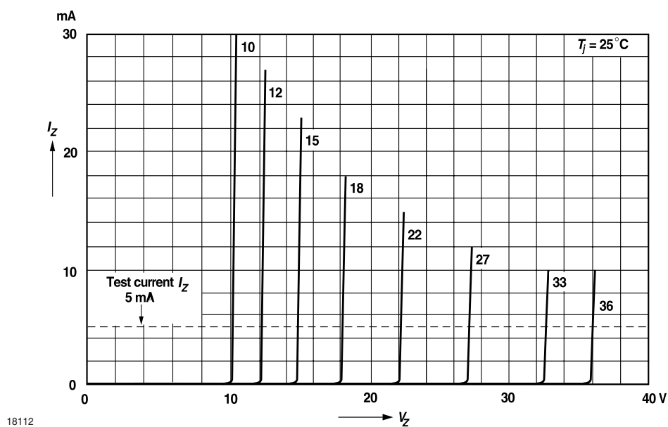
Figure 17. Breakdown Characteristics
