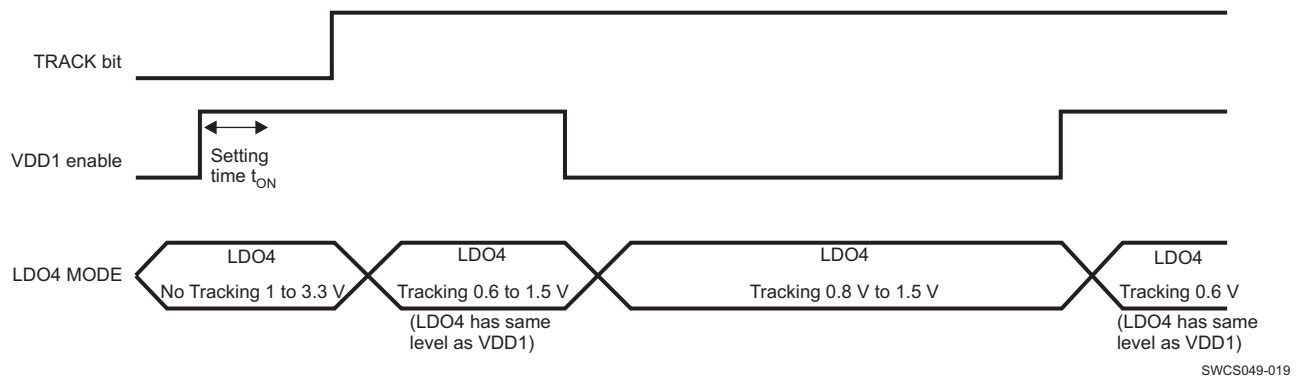
Figure 6-3. Tracking LDO
