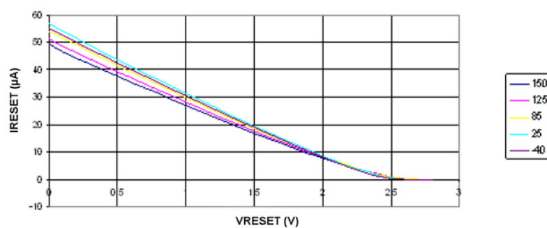
Figure 27-14. Reset Pull-up Resistor Current versus Reset Pin Voltage ( V_{CC} = 2.7V )
