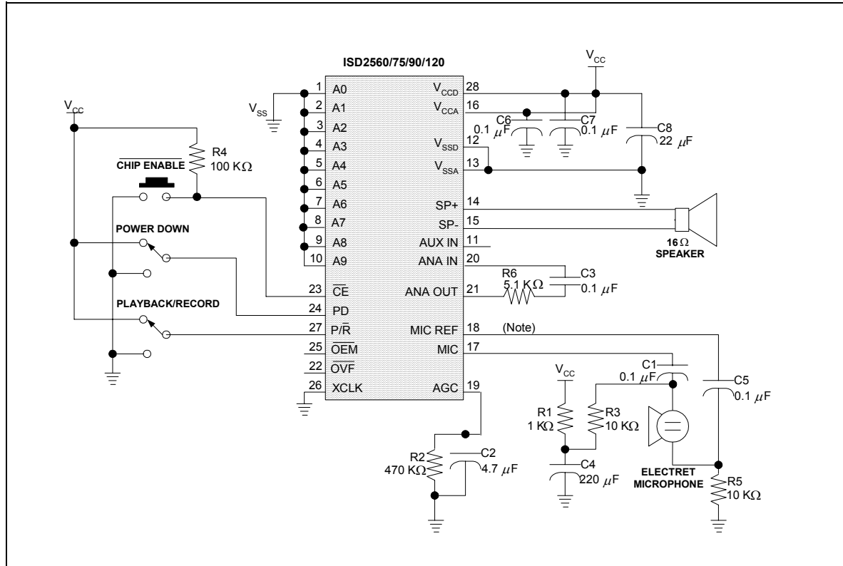
FIGURE 5: DESIGN SCHEMATIC
