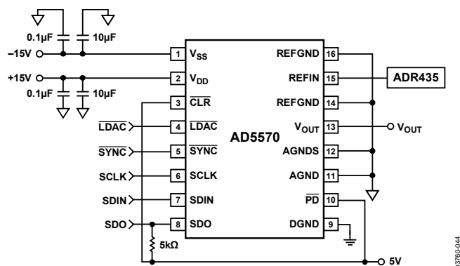
Figure 39. Typical Operating Circuit
