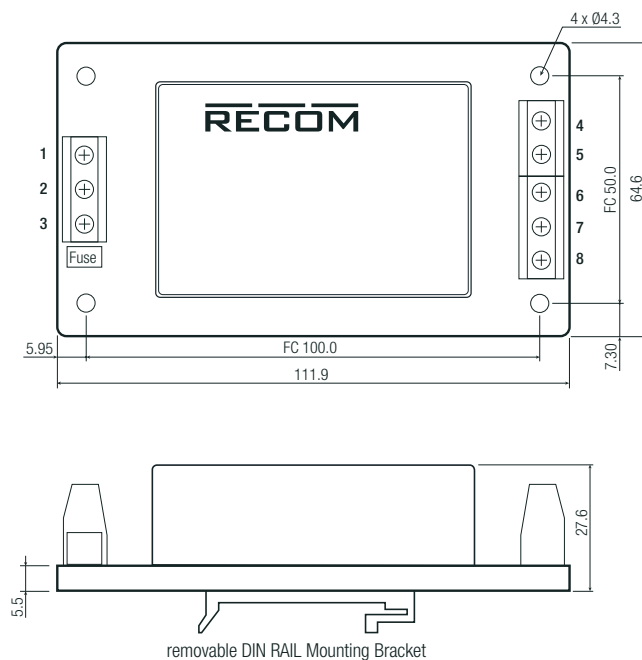
Screw Terminal Module "ST" version
