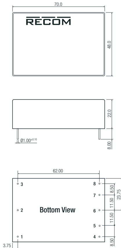
Dimension Drawing (mm)
