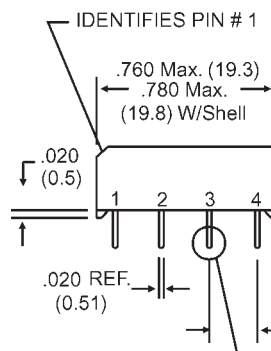
End View - 9081, 9081C & 9081C1
