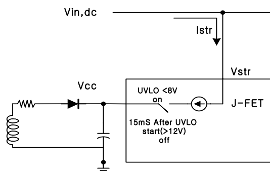
Figure 4. High voltage current source
