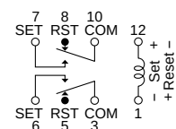
Schematic (Bottom view)
