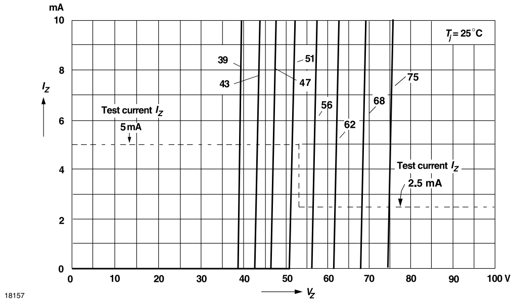
Figure 18. Breakdown Characteristics
