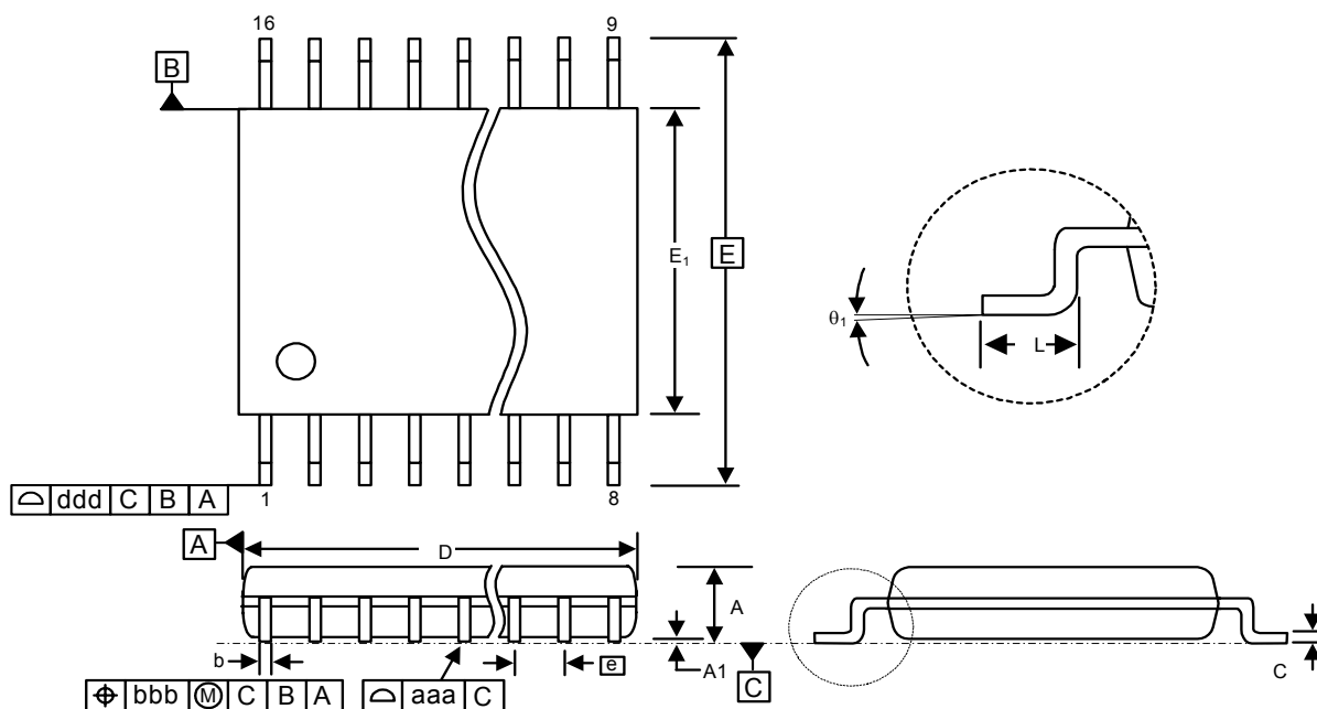
Figure 51. 16-Pin Thin Shrink Small Outline Package (TSSOP)
