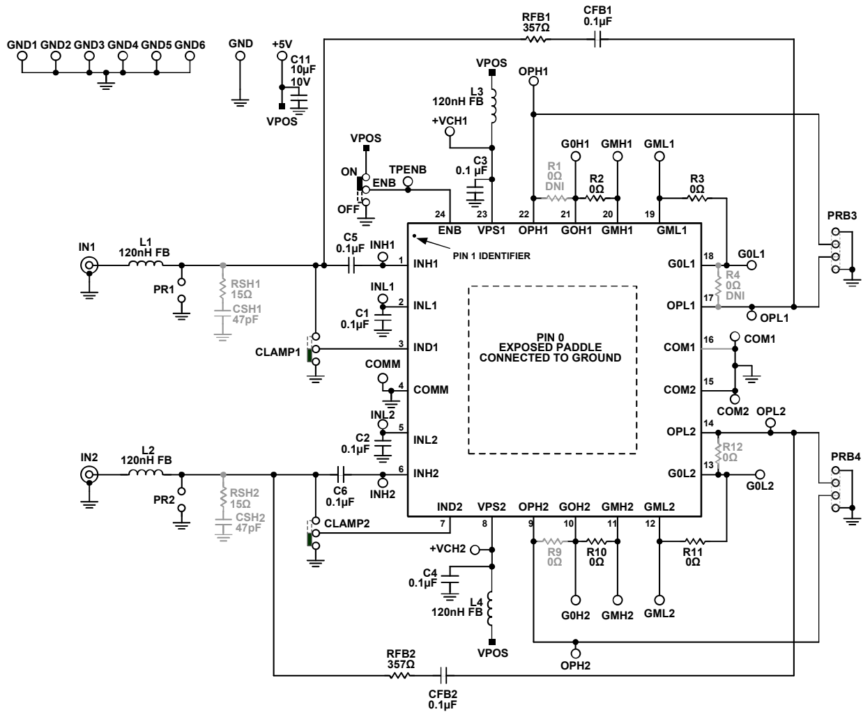
Figure 80. AD8432-EVALZ Schematic
