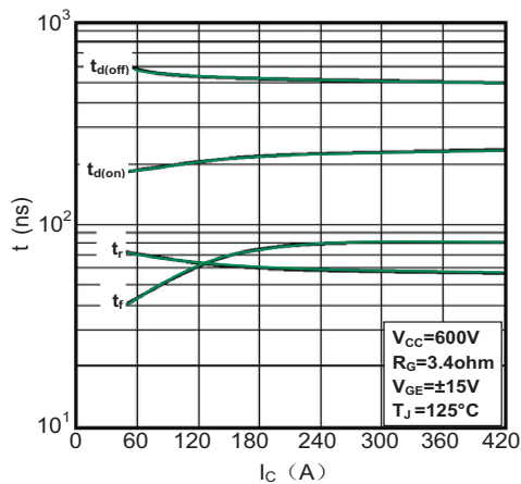
Figure 5: Switching Times vs. Collector Current
