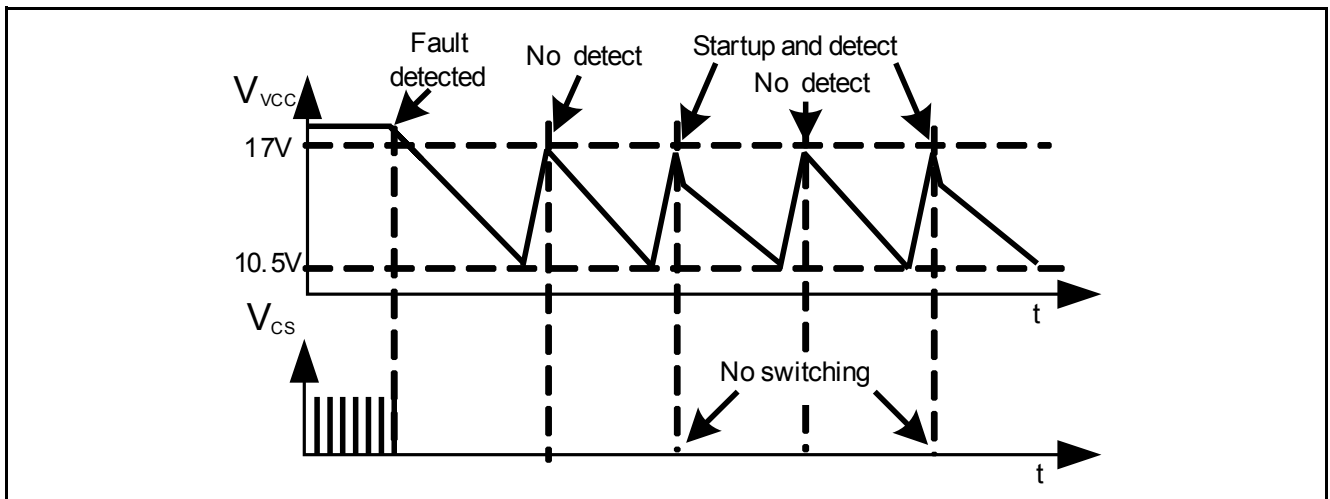
Figure 27 Nonswitch Auto Restart Waveform
