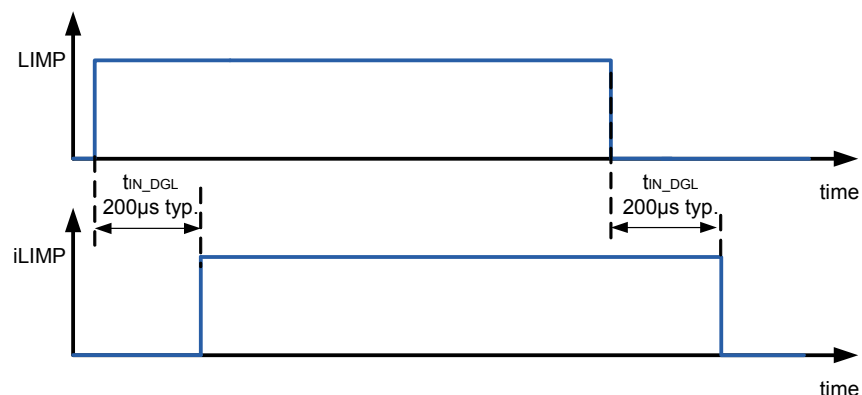
Figure 34. LIMP and iLIMP signal
