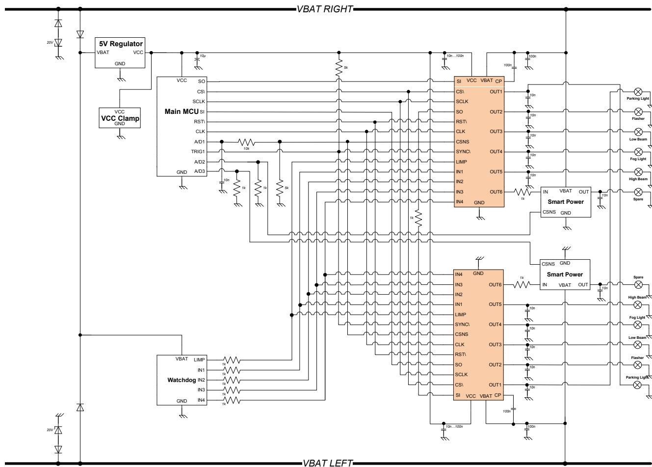
Figure 36. Typical front lighting application
