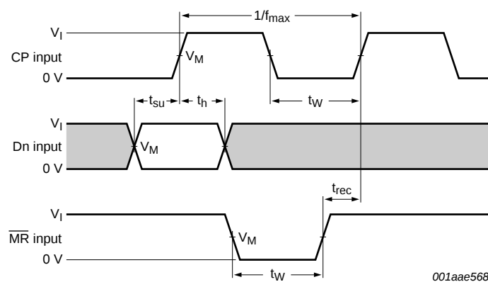
b. CP and \overline{\text{MR}} minimum pulse widths, \overline{\text{MR}} to CP recovery time, and Dn to CP set-up and hold times
