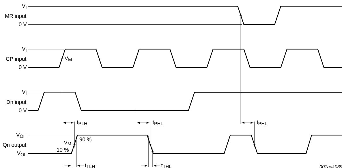
a. CP and \overline{\text{MR}} to Qn Propagation delays and Qn transition times
