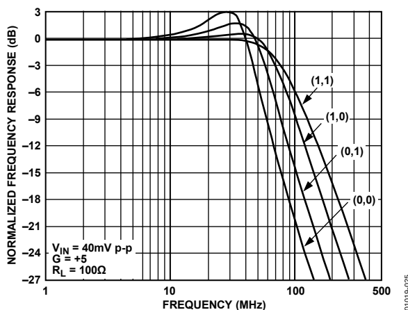
Figure 23. Frequency Response; V_S = \pm 12\text{ V} , @ PWDN1, PWDN0 Codes
