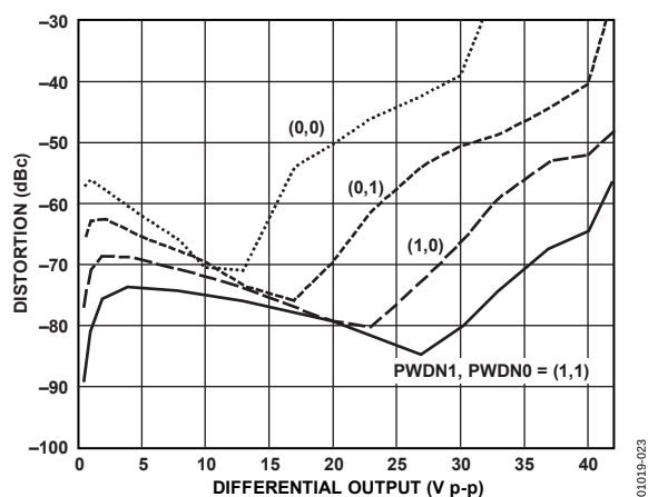
Figure 21. Distortion vs. Output Voltage; Third Harmonic, V_S = \pm 12\text{ V} , G = +10 , f = 1\text{ MHz} , R_L = 50\ \Omega , Differential
