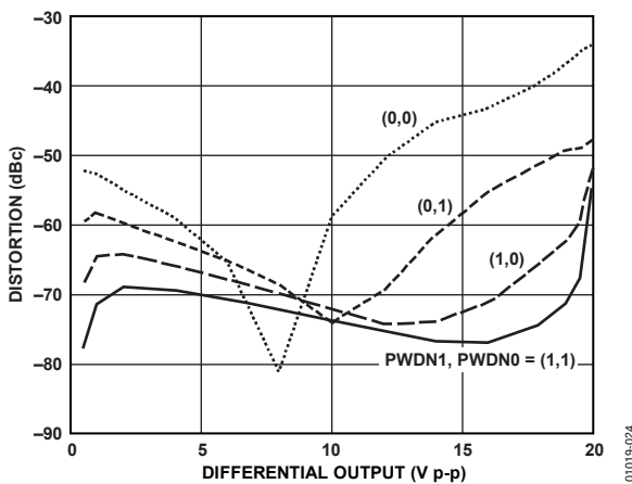
Figure 22. Distortion vs. Output Voltage; Third Harmonic, V_S = \pm 6\text{ V} , G = +10 , f = 1\text{ MHz} , R_L = 50\ \Omega , Differential
