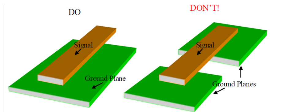
Figure 25. Recommended Shielding for Critical Signals.
