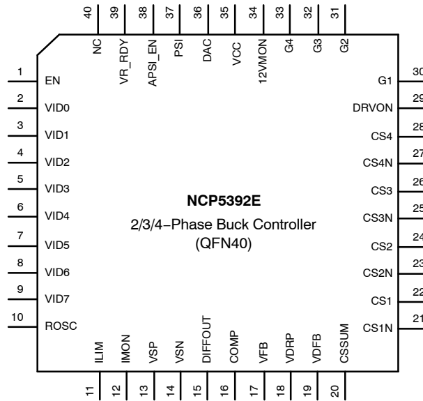
Figure 1. NCP5392E QFN40 Pin Connections (Top View)
