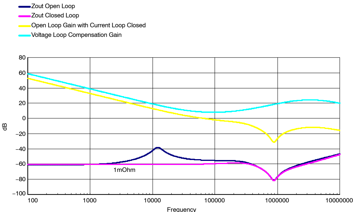
Figure 14. NCP5392E Circuit Frequency Response
