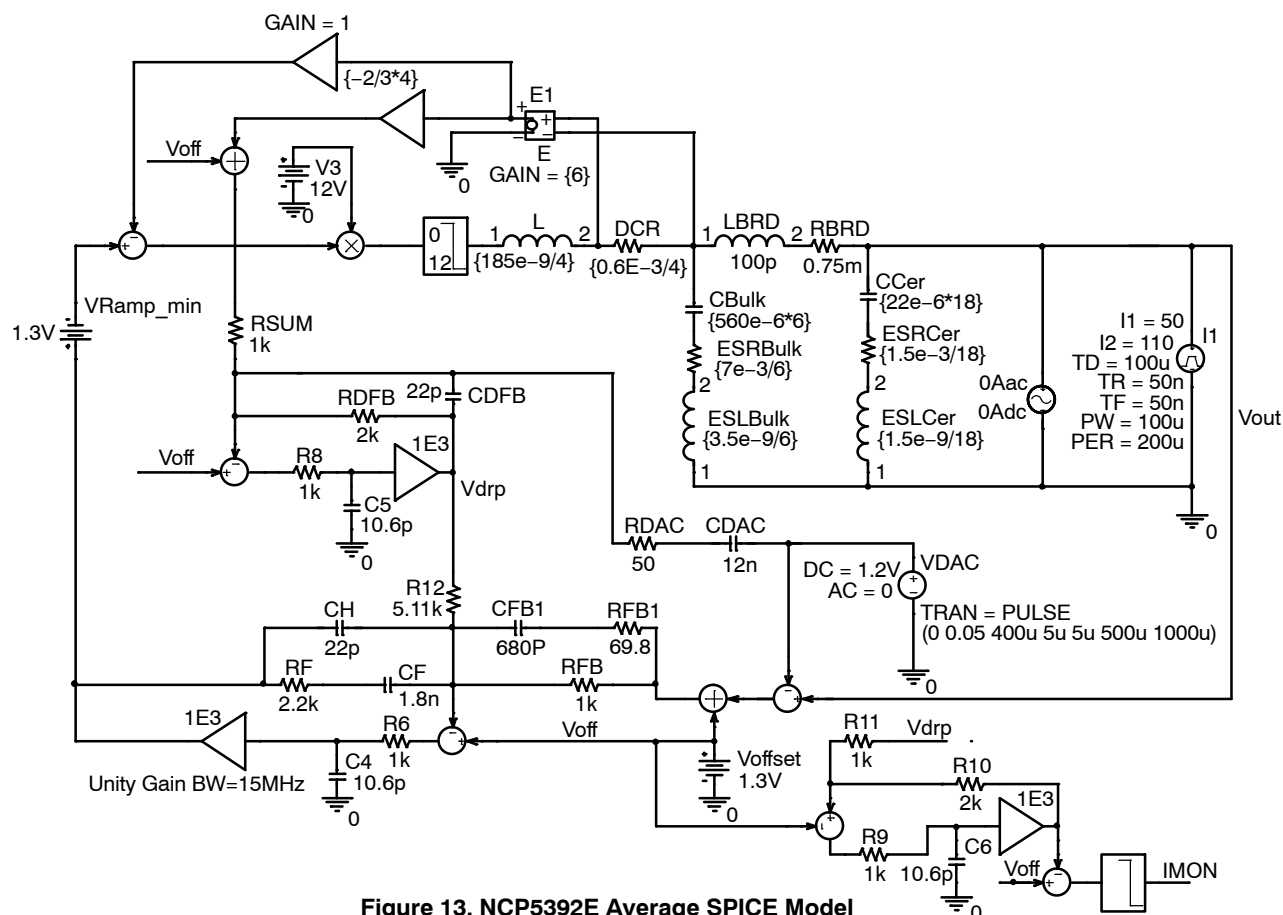
Figure 13. NCP5392E Average SPICE Model
