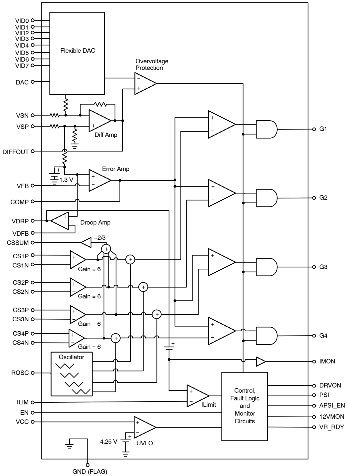
Figure 2. NCP5392E Block Diagram
