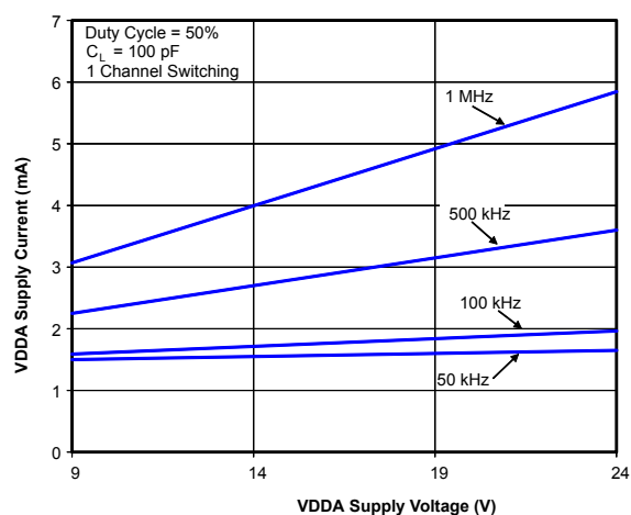
Figure 2.13. Supply Current vs. Supply Voltage
