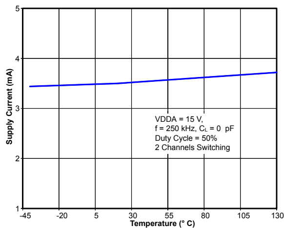
Figure 2.11. Supply Current vs. Temperature
