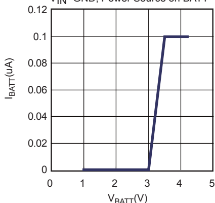
Battery Reverse Current I BATT vs V BATT Curve
