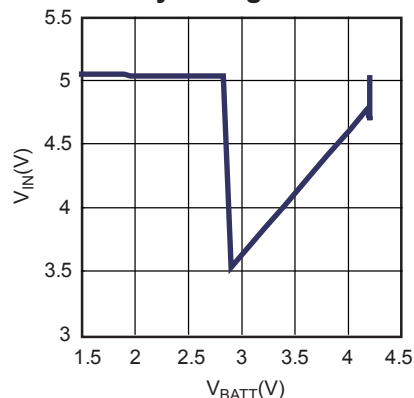
Charge Input Voltage vs Battery Voltage
