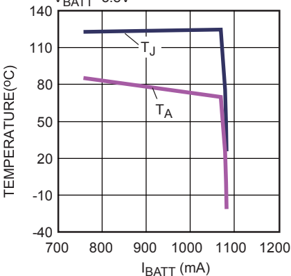
CC Charge Current vs. Temp
