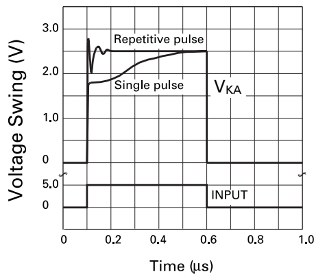
Pulse Response
