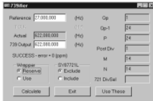
Figure 14. Generating 622.08MHz Without the Wrapper (Using SY87739L only)
