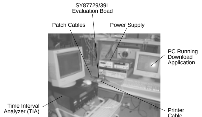
Figure 2. Test Set-Up with Internal Reference Oscillator
