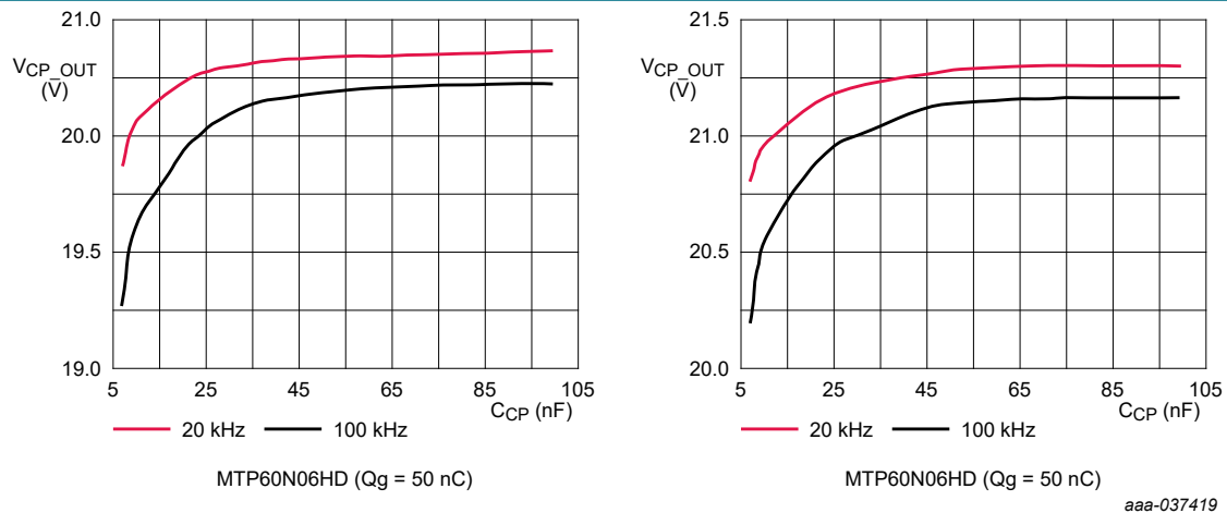
Figure 10. V_{CP\_OUT} Versus C_{CP}
