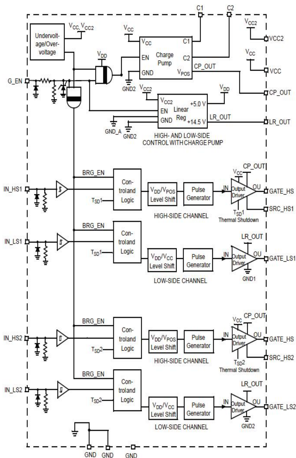
Figure 2. Internal block diagram
