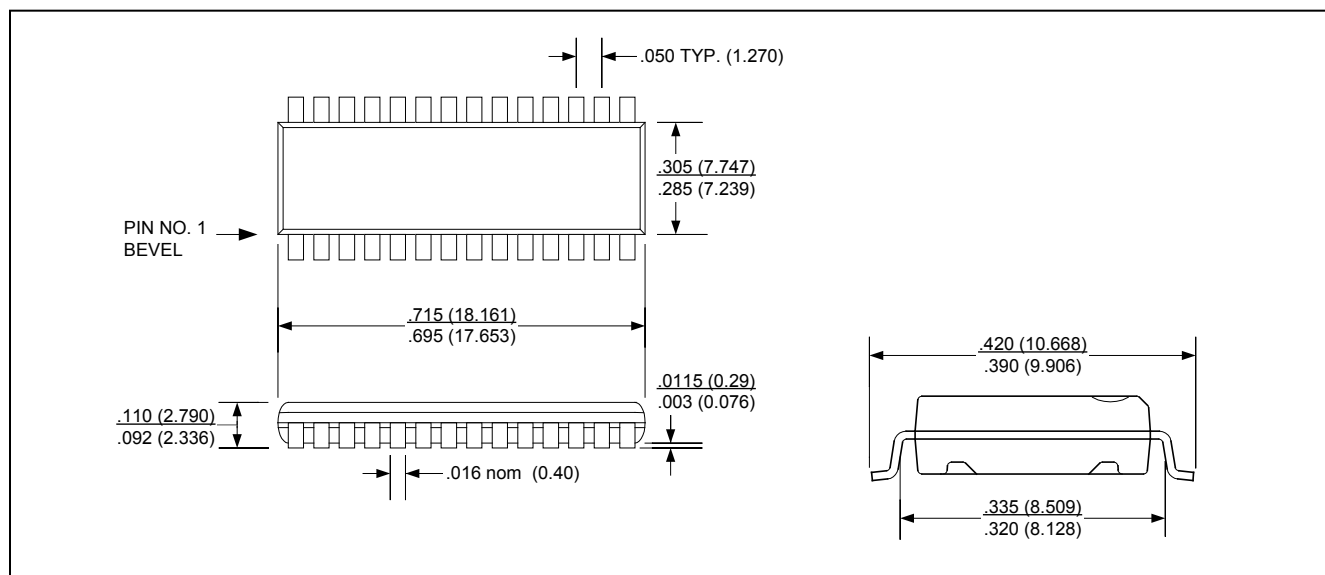
Figure 13: 28 Lead SO
