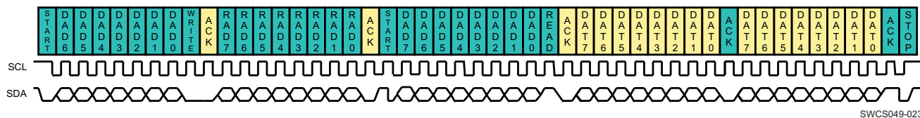
Figure 6-10. I²C Read Access Multiple Bytes
