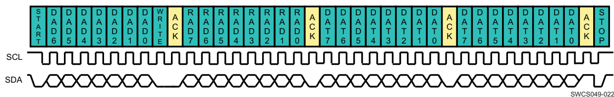
Figure 6-9. I²C Write Access Multiple Bytes
