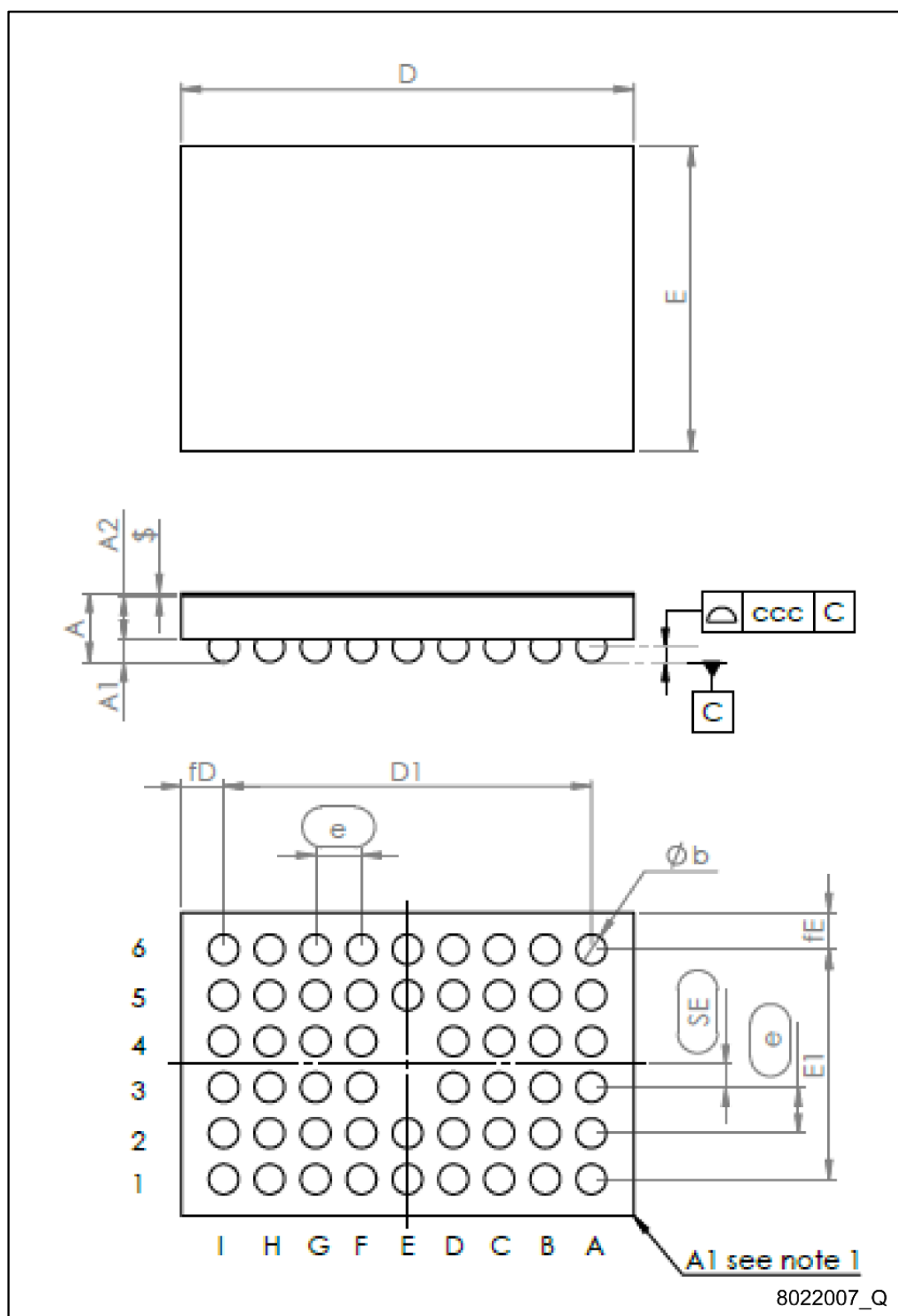
Figure 1: CSP (3.97x2.67 mm) package outline
