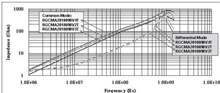
Impedance vs Frequency Characteristic:
