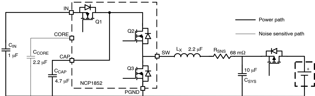
Figure 24. NCP1852 Power Path
