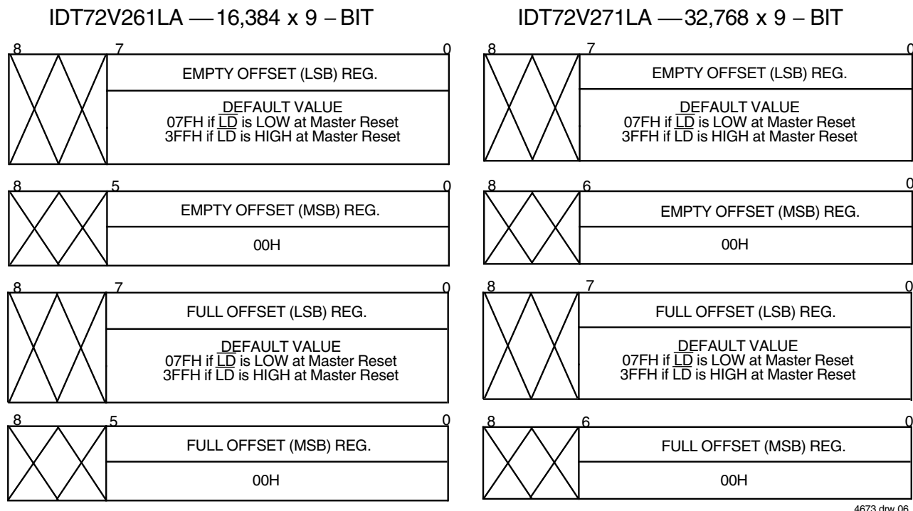
Figure 3. Offset Register Location and Default Values
