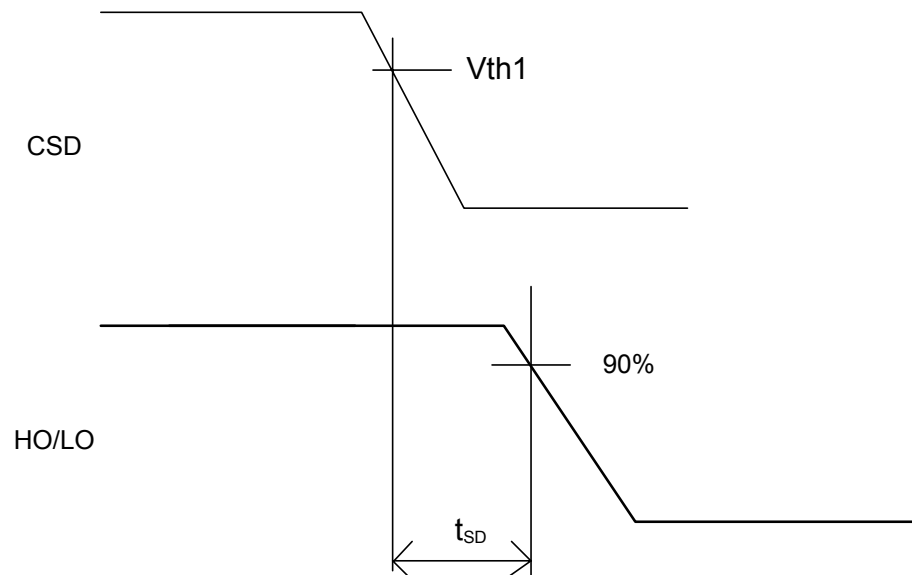
Figure 2: CSD to Shutdown Waveform Definitions
