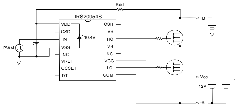
Figure 18: Supplying V_{DD}
