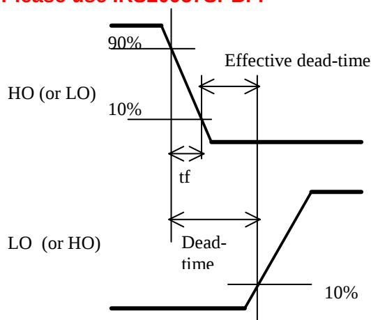
Figure 15: Effective Deadtime
