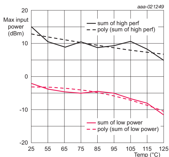
Fig 54. Maximum input level
