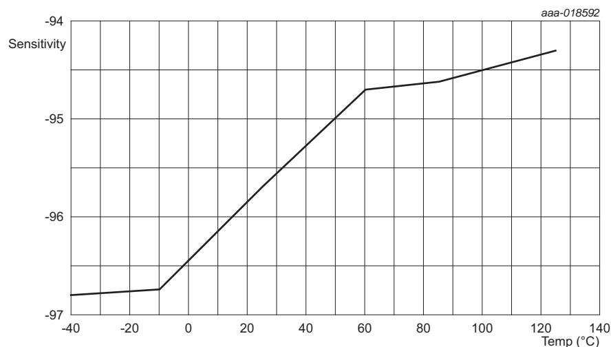
Fig 53. Typical receiver sensitivity versus temperature
