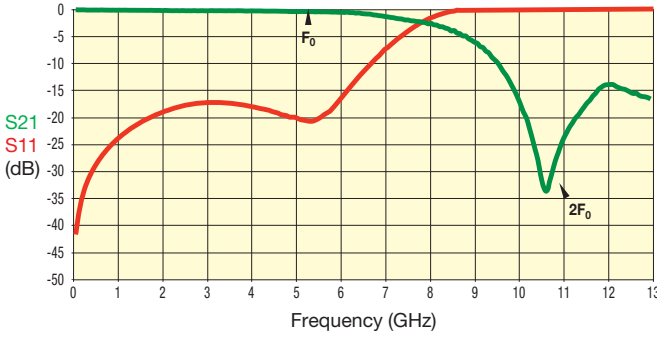
LP0603N5500ANTR
