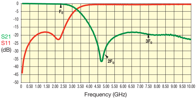
LP0603A2442ANTR
