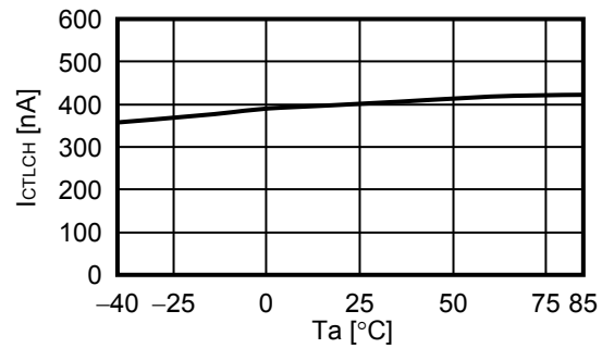
4.1 I_{CTLCH} vs. T_a ( V_{DS} = 3.5 V)
