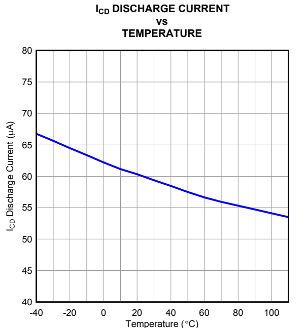
Figure 3. I_{CD} Discharge Current
