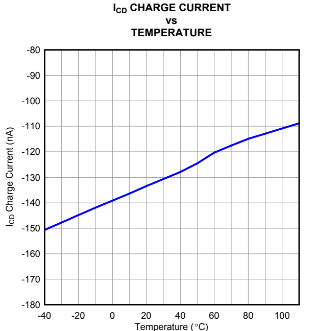
Figure 2. I_{CD} Charge Current
