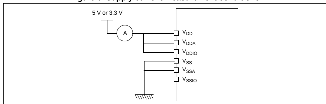
Figure 6. Supply current measurement conditions
