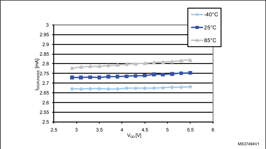
Figure 11. Typ. I_{DD(RUN)} vs V_{DD} , HSE user external clock, f_{CPU} = 16 MHz
