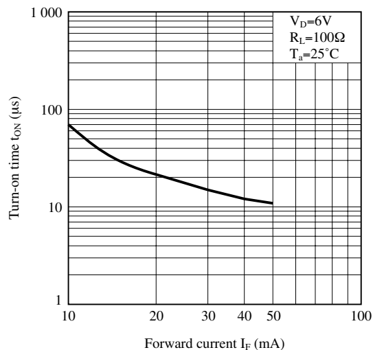
Fig.8-a Turn-on Time vs. Forward Current (S101DH1)
