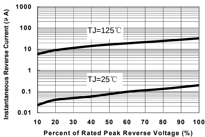
Fig.3-Typical Reverse Characteristics
