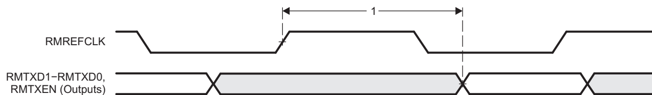
Figure 9-15. EMAC Transmit Interface Timing RMI Operation
