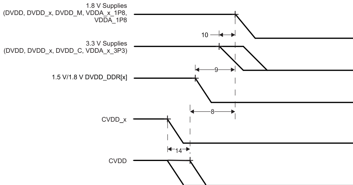
Figure 8-2. Power-Down Sequence
