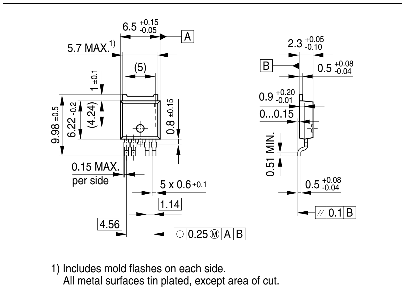
Figure 1 PG-T0252-5-11 (Plastic Dual Small Outline Package) (RoHS-compliant)
