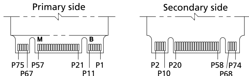
Figure 4: Interface Connections – M.2 Type 2280
